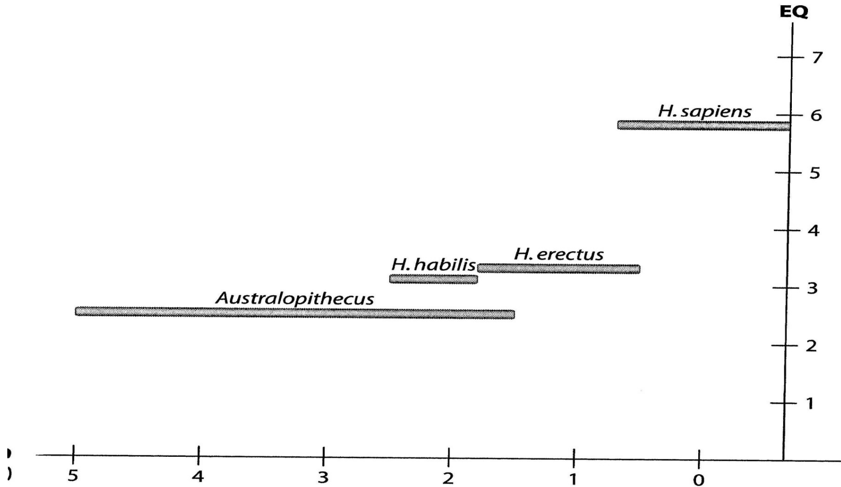
Figure 10.2: Hominid Encephalization Quotients
